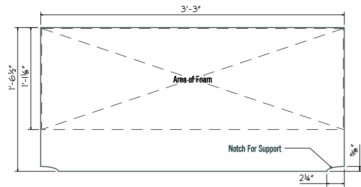
Front Bench Seat Back 1/2" thick
