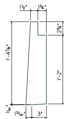
Left Bench Support Cover Piece 1/4" thick
