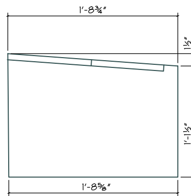
Left Bench Support (Side View) 3/4" thick (Orig 1/2" ?)
