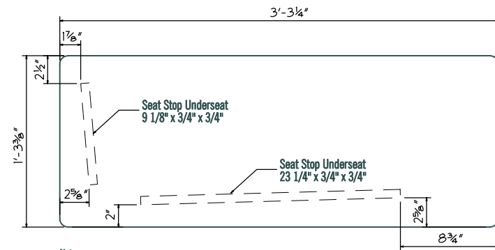
Front Bench Seat Top View 1/2" thick
