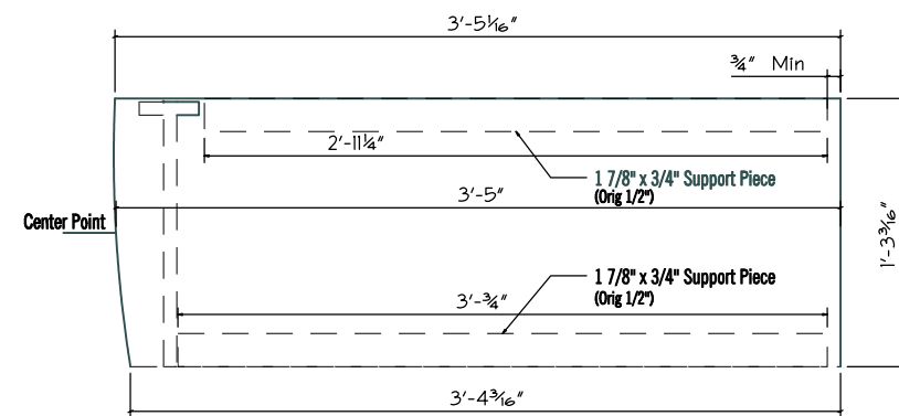
Under Front Seat 1/4" thick
